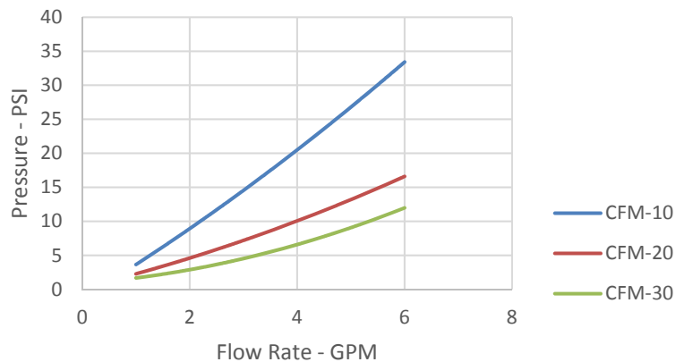
CFM 10, 20 & 30 Filters
